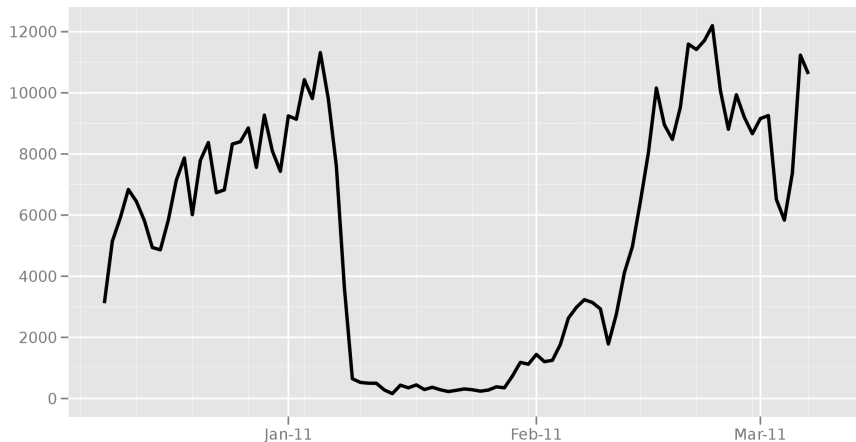
Directly connecting Iranian Tor users
